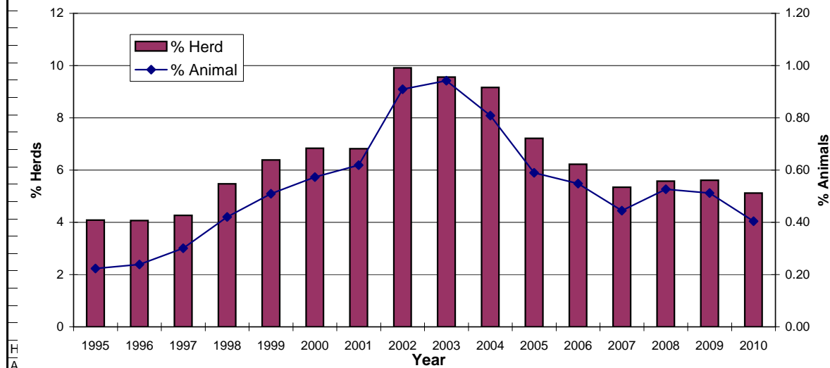
TB herd and animal incidence: 1995 to 2010
