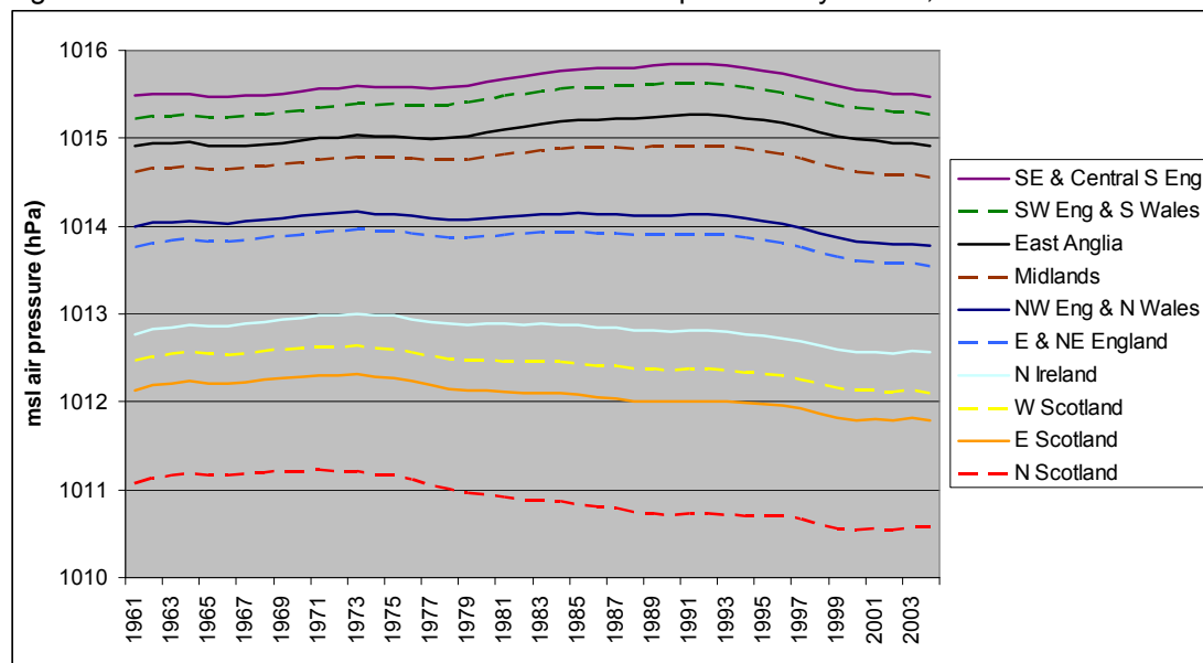
Figure 16: Kernel smoothed annual mean sea level pressure by district, 1961-2004
