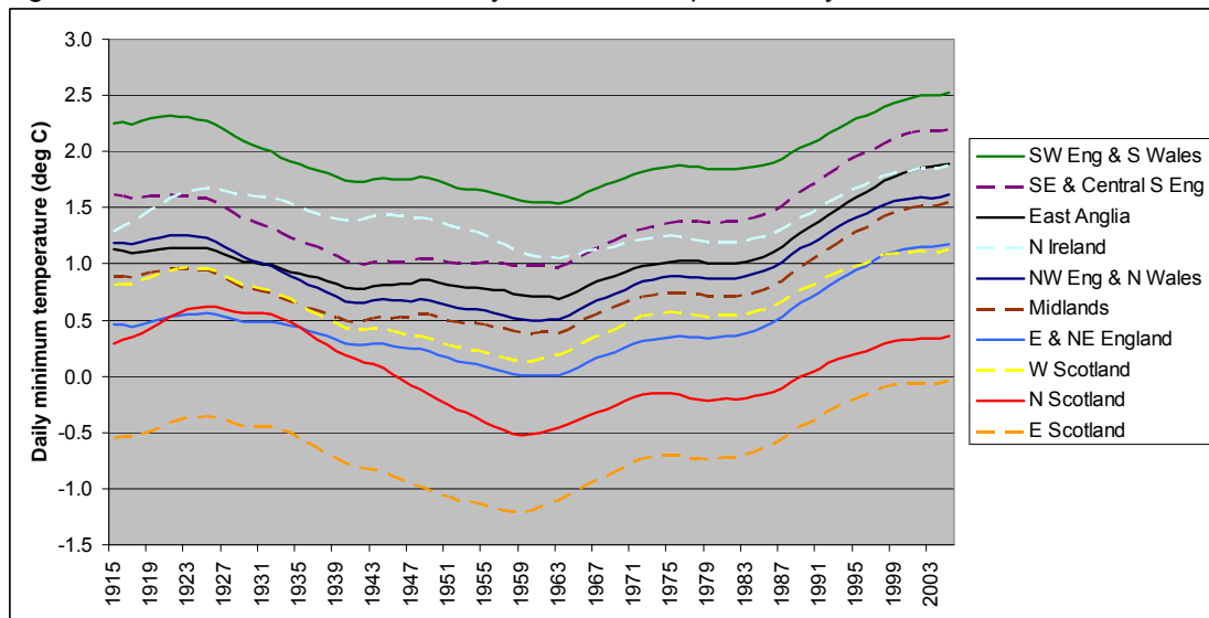
Figure 5: Kernel smoothed winter daily minimum temperature by district, 1914-2004.
