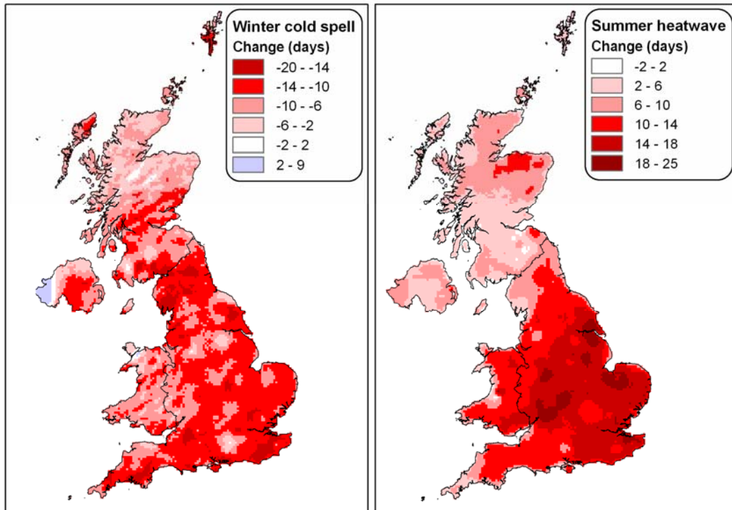
Map 6: Gridded trends for winter half-year cold spell duration and summer half-year heat wave duration, showing the change (in days) from 1961 to 2003
