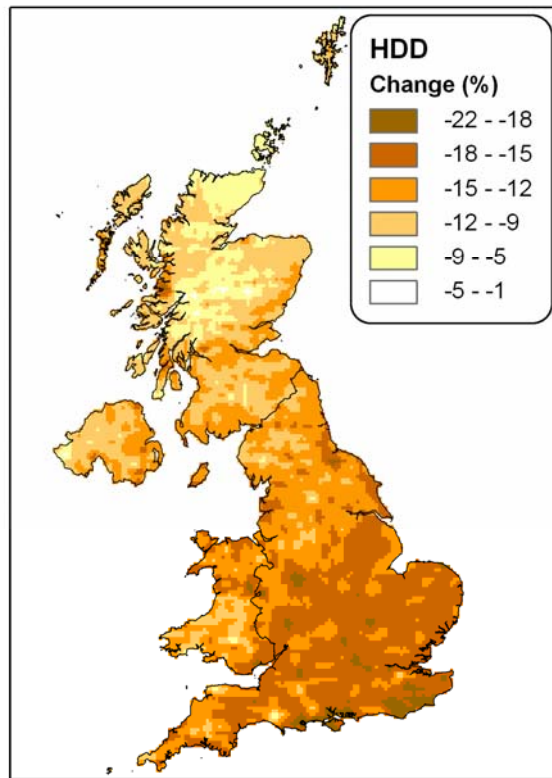
Map 4: Gridded trends for heating degree days (HDD), showing the percentage change from 1961 to 2003.
