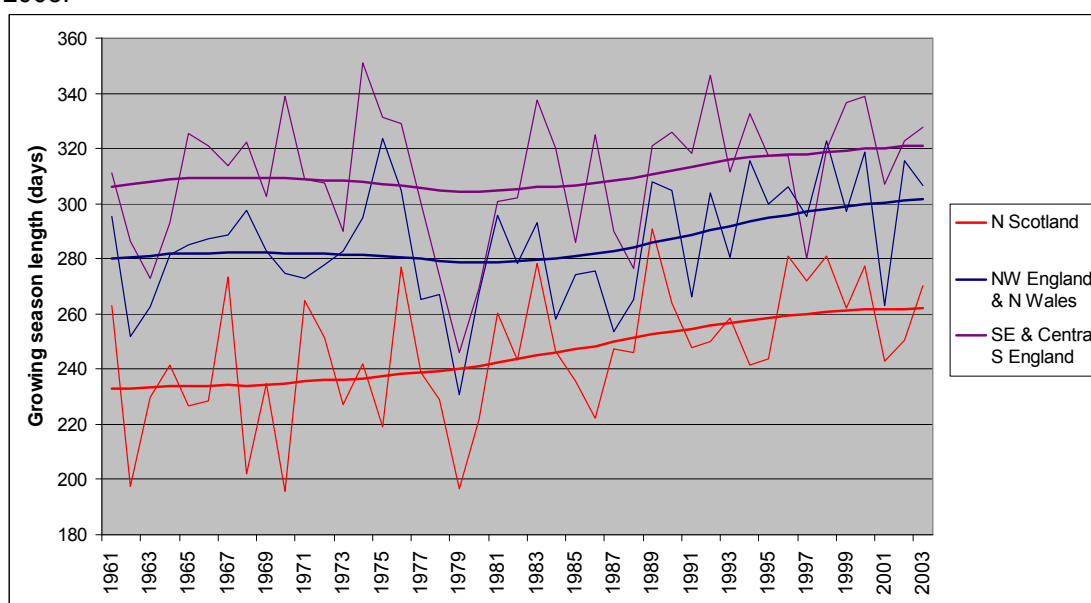
Figure 7: Actual and kernel smoothed growing season length (days) for three districts, 1961-2003.
