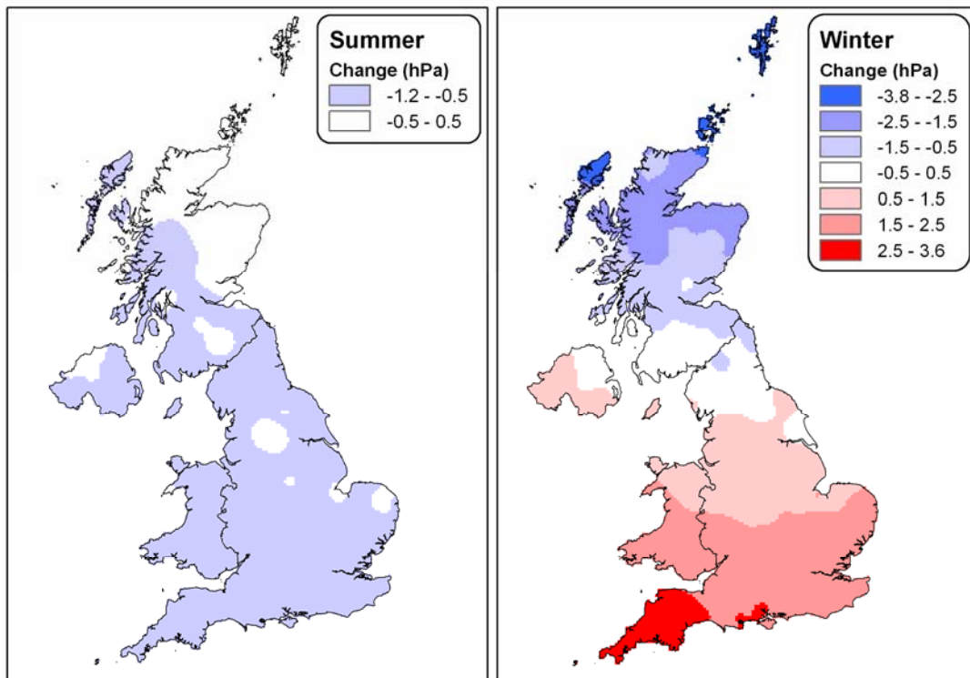
Map 11: Gridded trends for mean sea level pressure, showing the change (in hPa) from 1961 to 2004; a) summer, b) winter.
