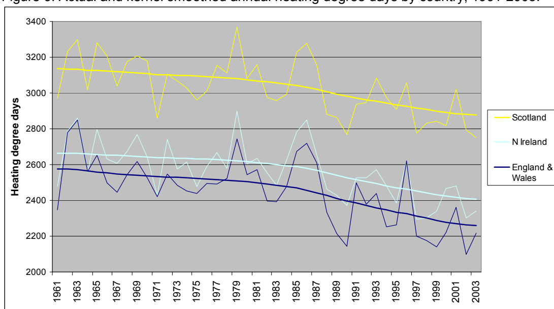
Figure 6: Actual and kernel smoothed annual heating degree days by country, 1961-2003.
