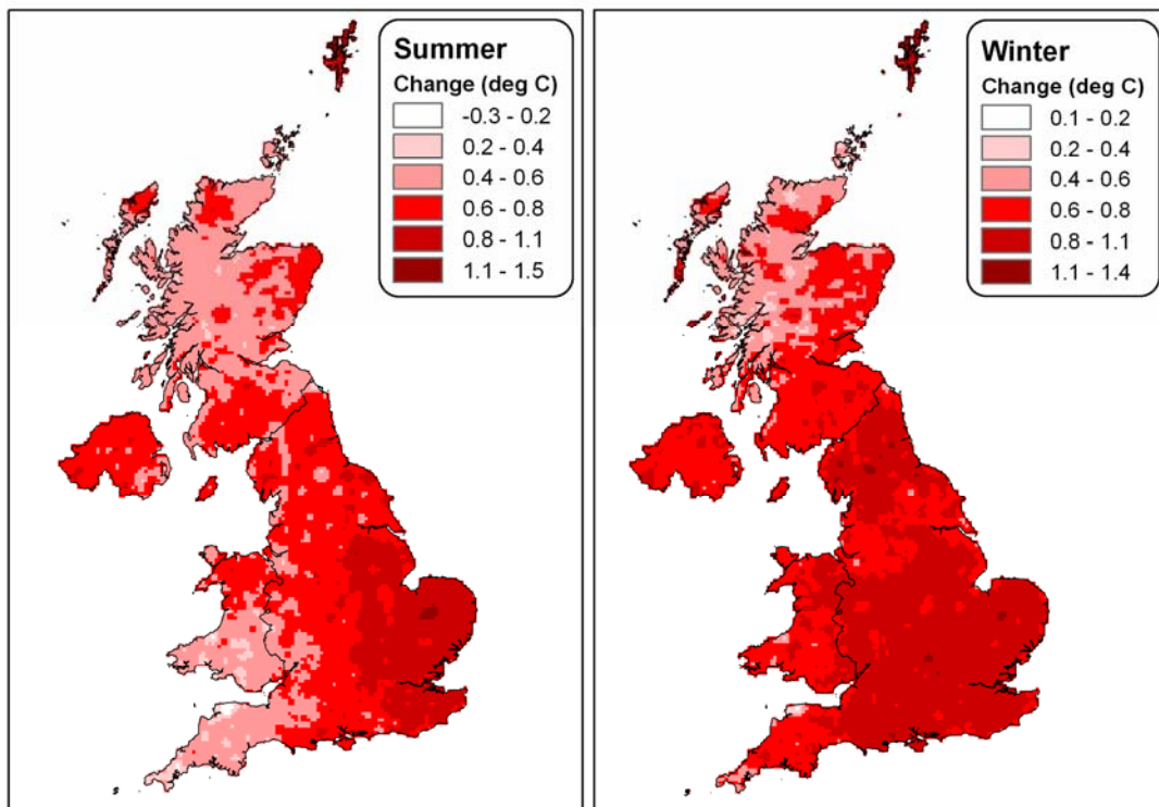
Map 3: 24-hour minimum temperature changes (°C) from the 1961-1990 average to 1991-2004; a) summer, b) winter.
