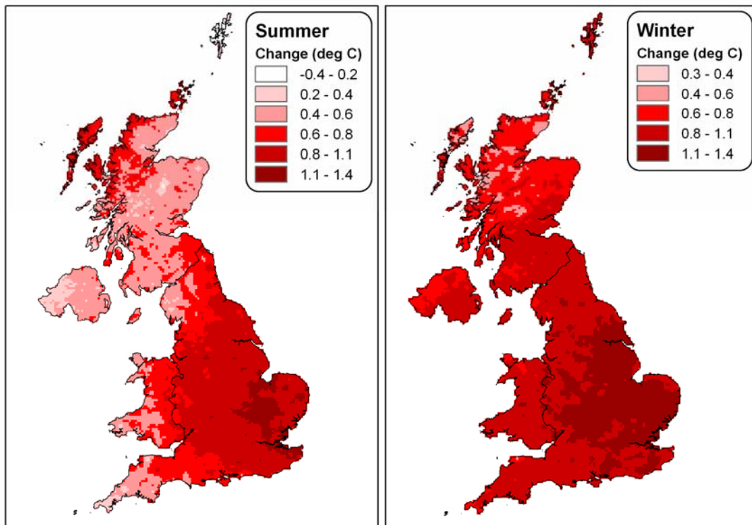
Map 2: 24-hour maximum temperature changes (°C) from the 1961-1990 average to 1991-2004; a) summer, b) winter.
