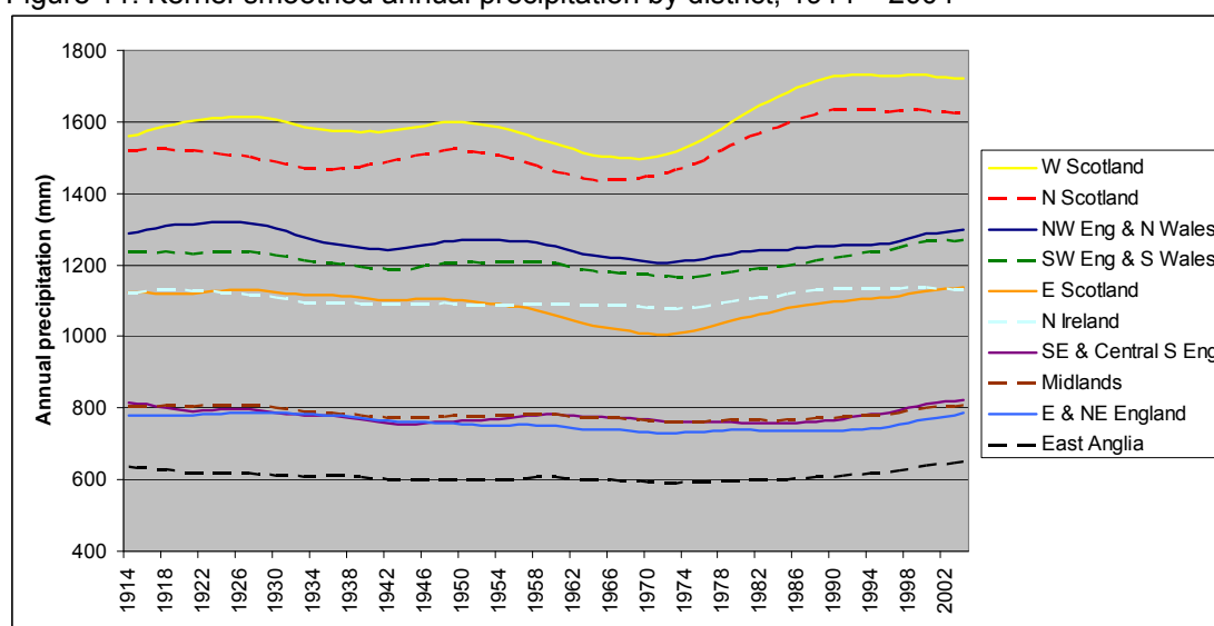
Figure 11: Kernel-smoothed annual precipitation by district, 1914 – 2004
