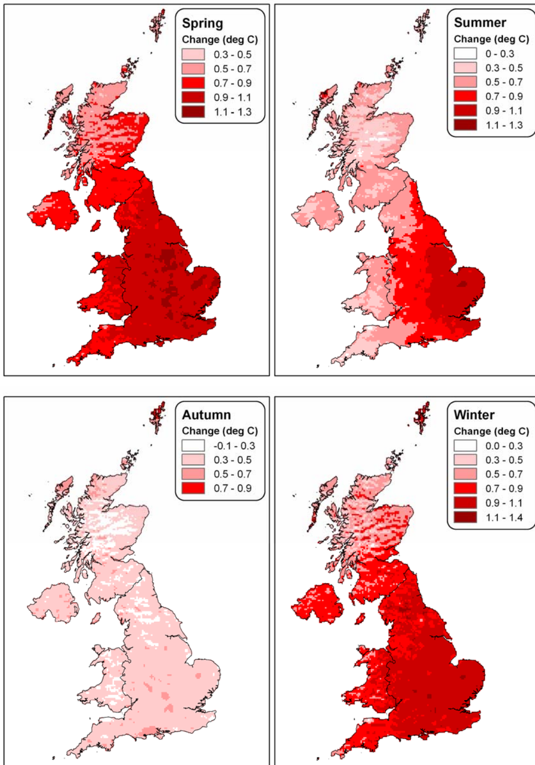
Map 1: Mean temperature change (°C) from the 1961-1990 average to 1991-2004; a) spring, b) summer, c) autumn, d) winter.
