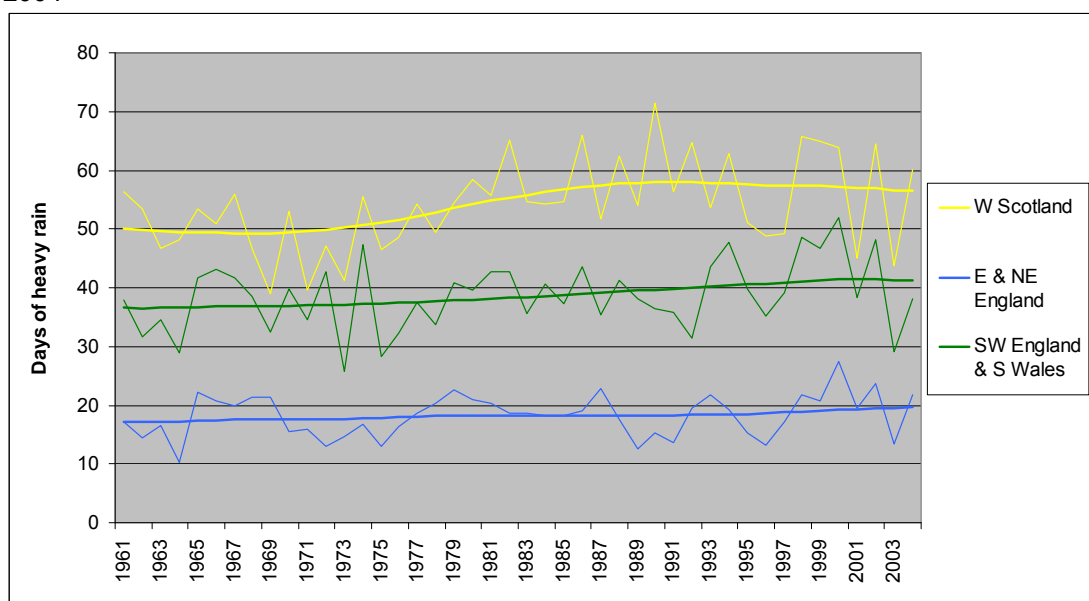
Figure 12: Actual and kernel-smoothed annual days of rain \geq 10 mm for three districts, 1961 – 2004
