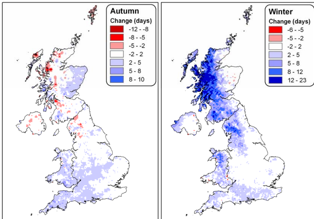
Map 8: Gridded trends for days of heavy rain \geq 10 mm, showing the change (in days) from 1961 to 2004; a) autumn, b) winter
