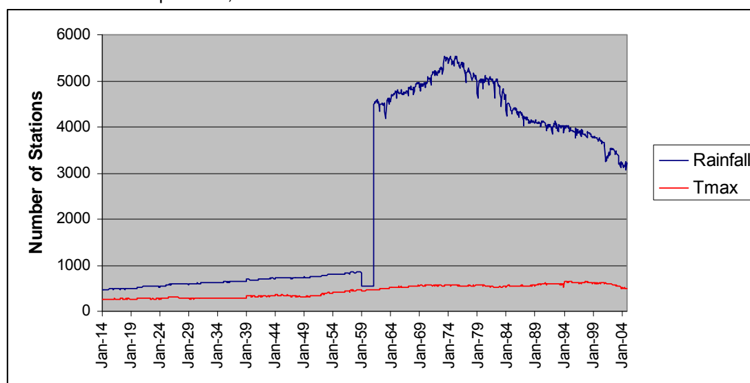
Figure 1: The number of stations used to create monthly gridded datasets for UK Precipitation and Maximum Temperature, 1914 – 2004.
