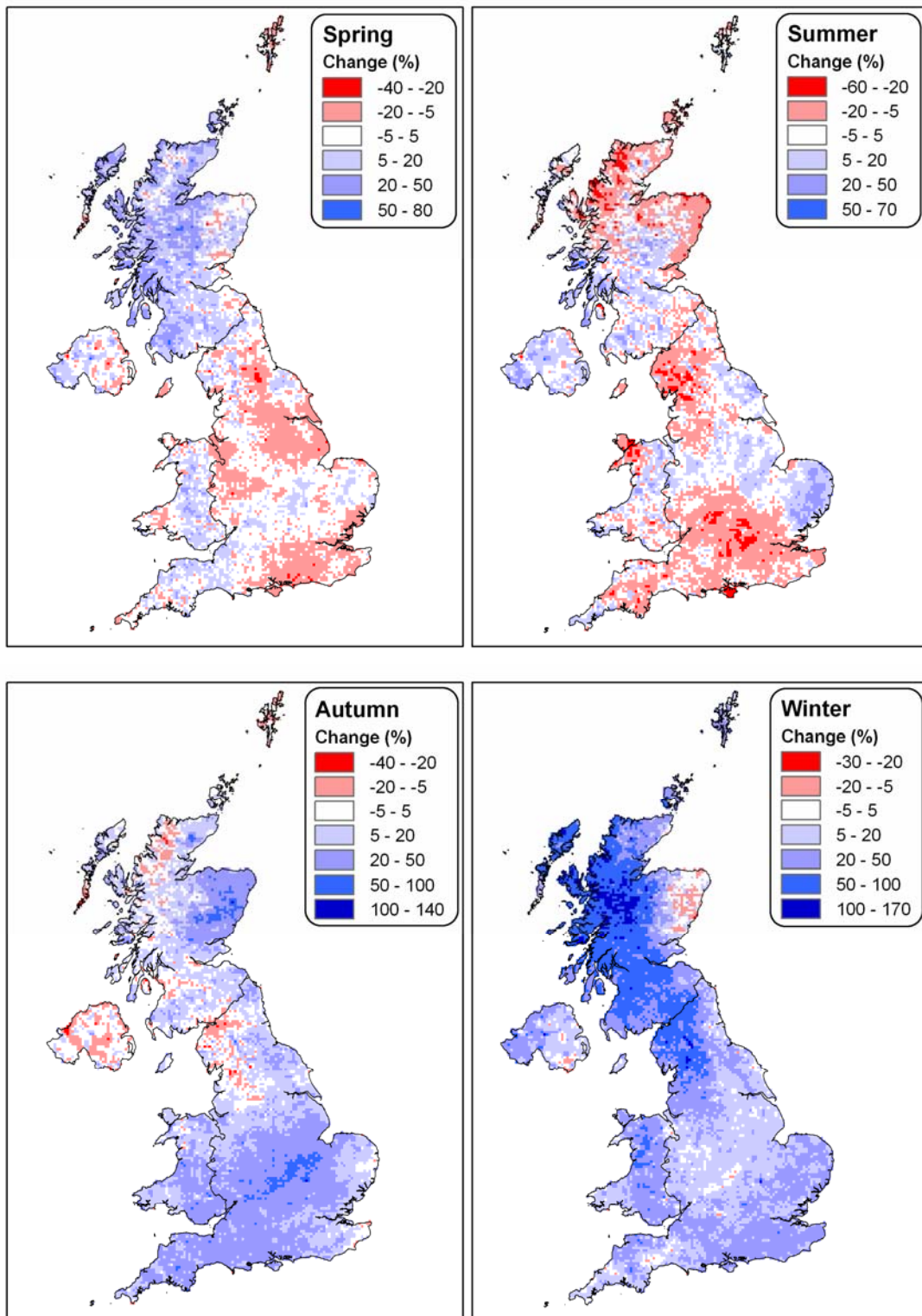
Map 7: Precipitation gridded trends, showing the percentage change from 1961 to 2004; a) spring, b) summer, c) autumn, d) winter.
