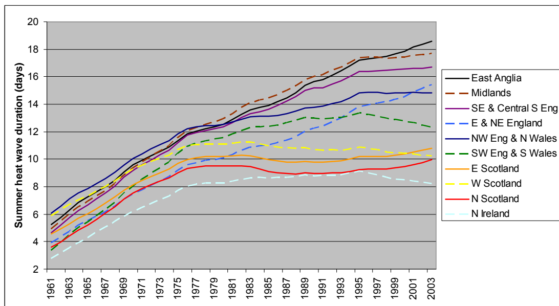
Figure 9: Kernel smoothed summer half-year heat wave duration (days) by district, 1961-2003.
