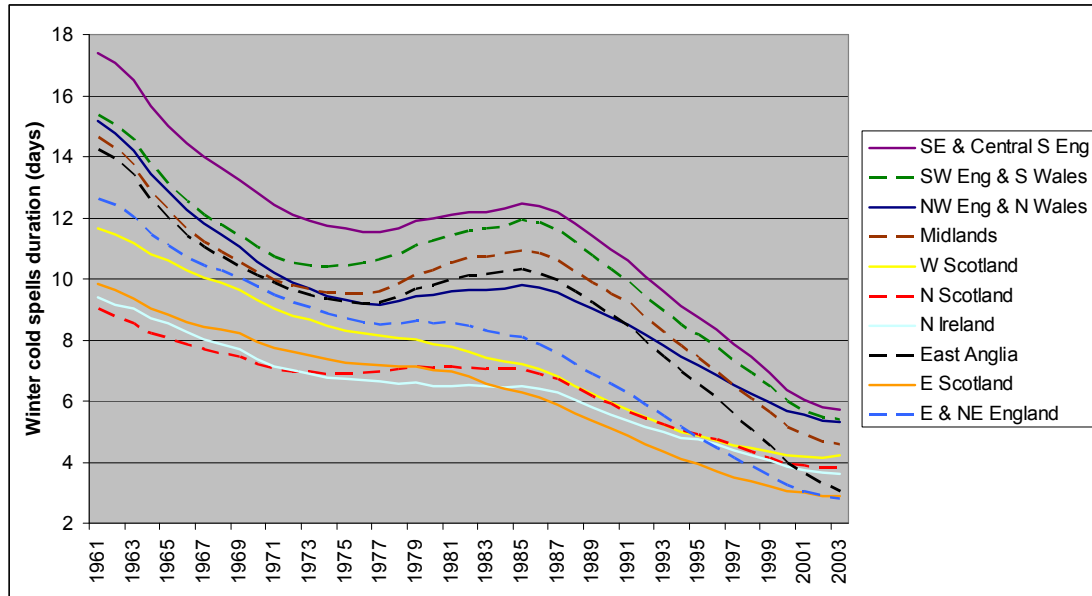
Figure 8: Kernel smoothed winter half-year cold wave duration (days) by district, 1961-2003.
