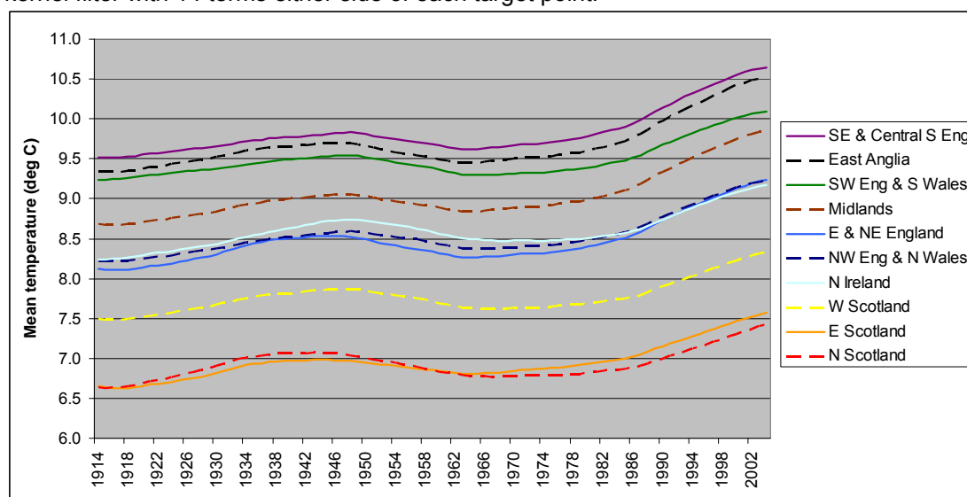
Figure 3: Annual mean temperature from 1914 to 2004 by district, smoothed with a triangular kernel filter with 14 terms either side of each target point.
