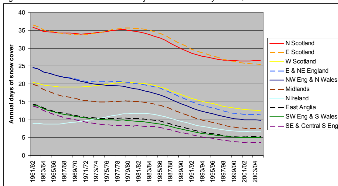
Figure 13: Kernel-smoothed annual days of snow cover by district, 1961/62 – 2004/05
