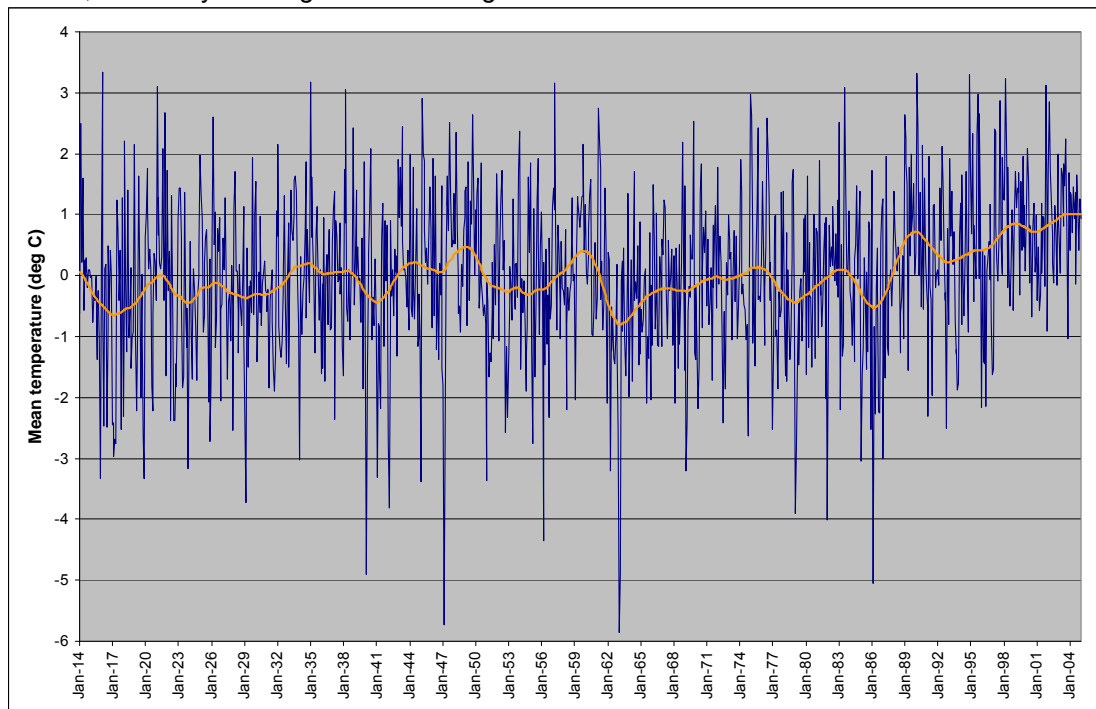
Figure 2: De-seasonalised time series of monthly mean temperature areally averaged over the UK, with a 5-year weighted smoothing filter.
