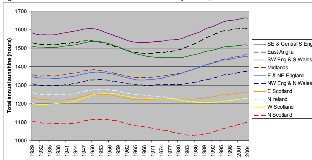
Figure 15: Kernel smoothed annual sunshine hours by district, 1929 – 2004.
