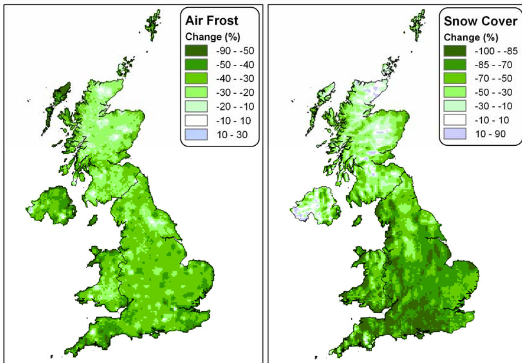
Map 9: Gridded trends for days of air frost and days of snow cover, showing the percentage change from 1961/62 to 2004/05.
