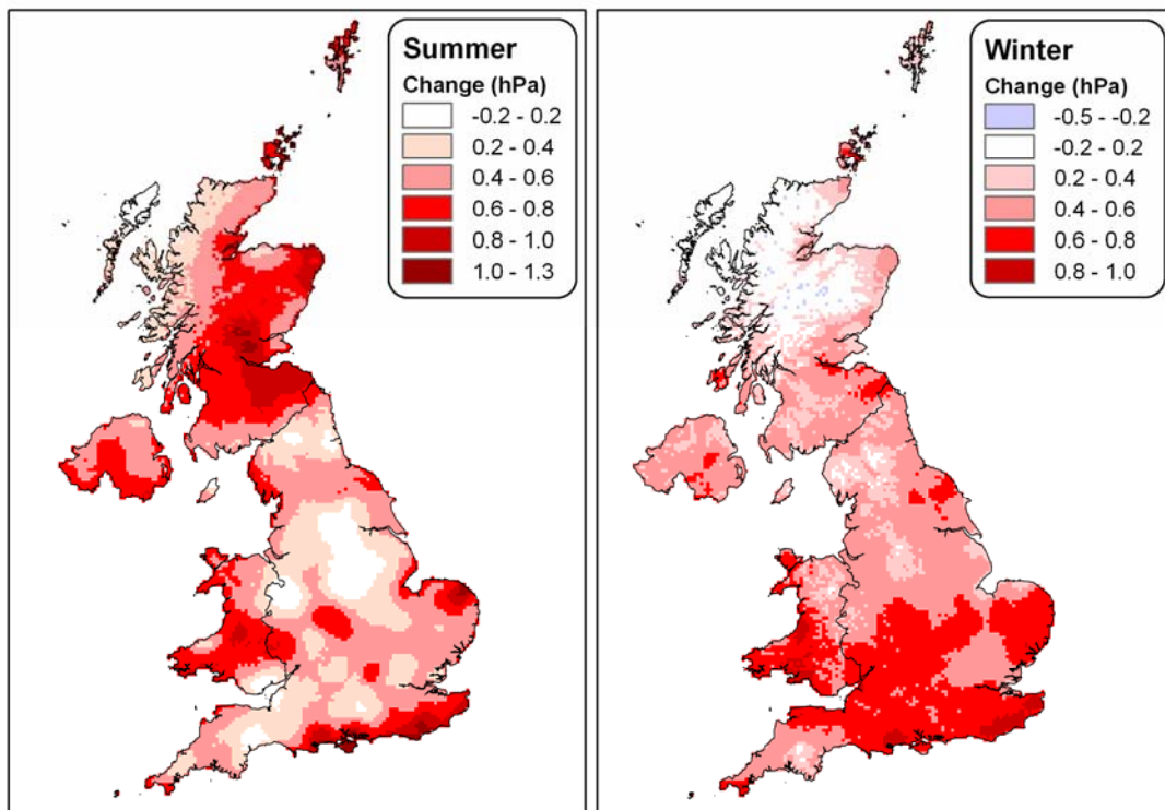
Map 12: Vapour pressure gridded trends, showing the change (in hPa) from 1961 to 2004; a) summer, b) winter.
