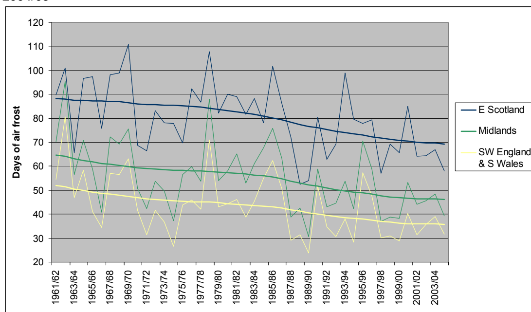
Figure 14: Actual and kernel-smoothed annual days of air frost for three districts, 1961/62 – 2004/05
