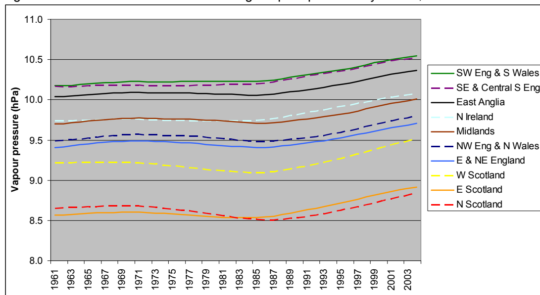
Figure 17: Kernel smoothed annual average vapour pressure by district, 1961-2004
