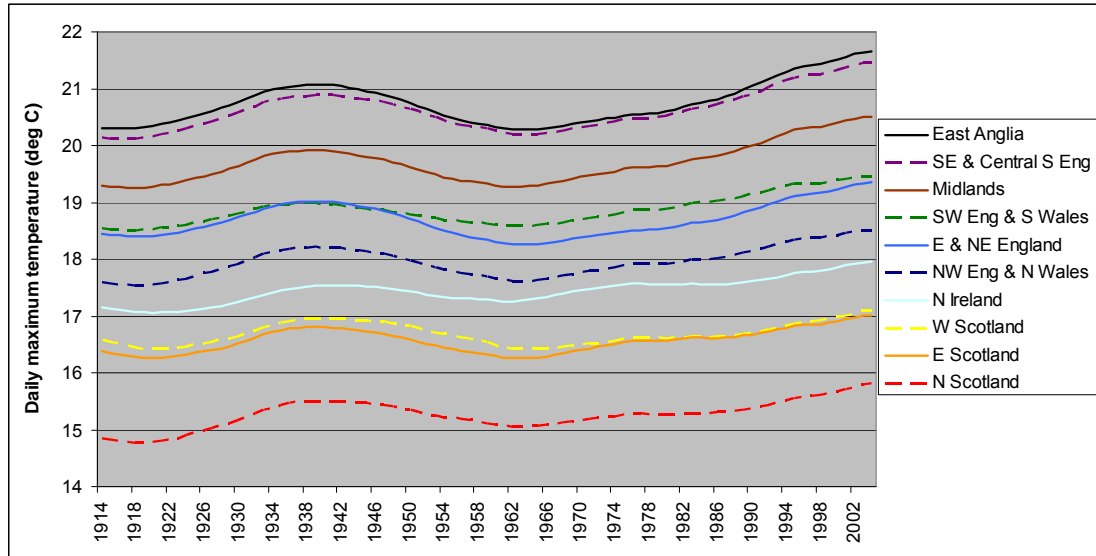
Figure 4: Kernel smoothed summer daily maximum temperature by district, 1914-2004.
