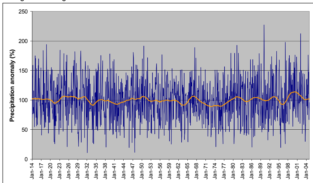
Figure 10: De-seasonalised monthly time series of UK precipitation with a 5-year weighted average smoothing filter
