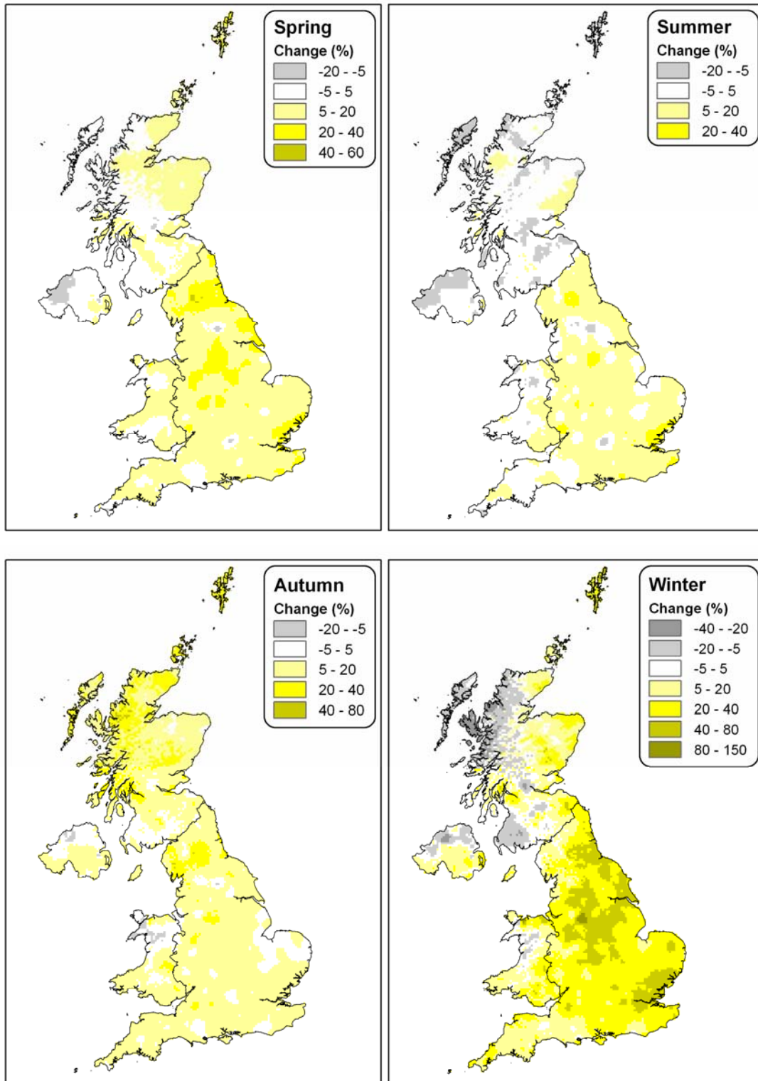
Map 10: Sunshine gridded trends, showing the percentage change from 1961 to 2004; a) spring, b) summer, c) autumn, d) winter.
