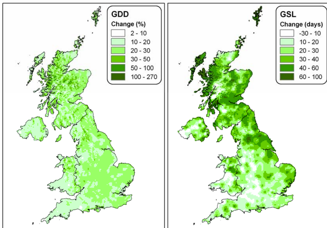
Map 5: Gridded trends for growing degree days (GDD) as a percentage, and growing season length (GSL) in days, showing the change from 1961 to 2003.
